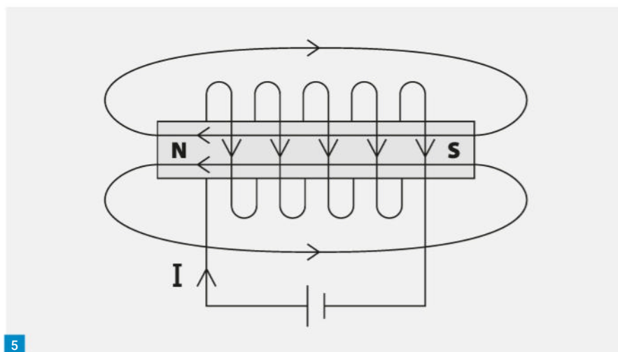
Fig. 5: Conductor wound around magnetic material.
